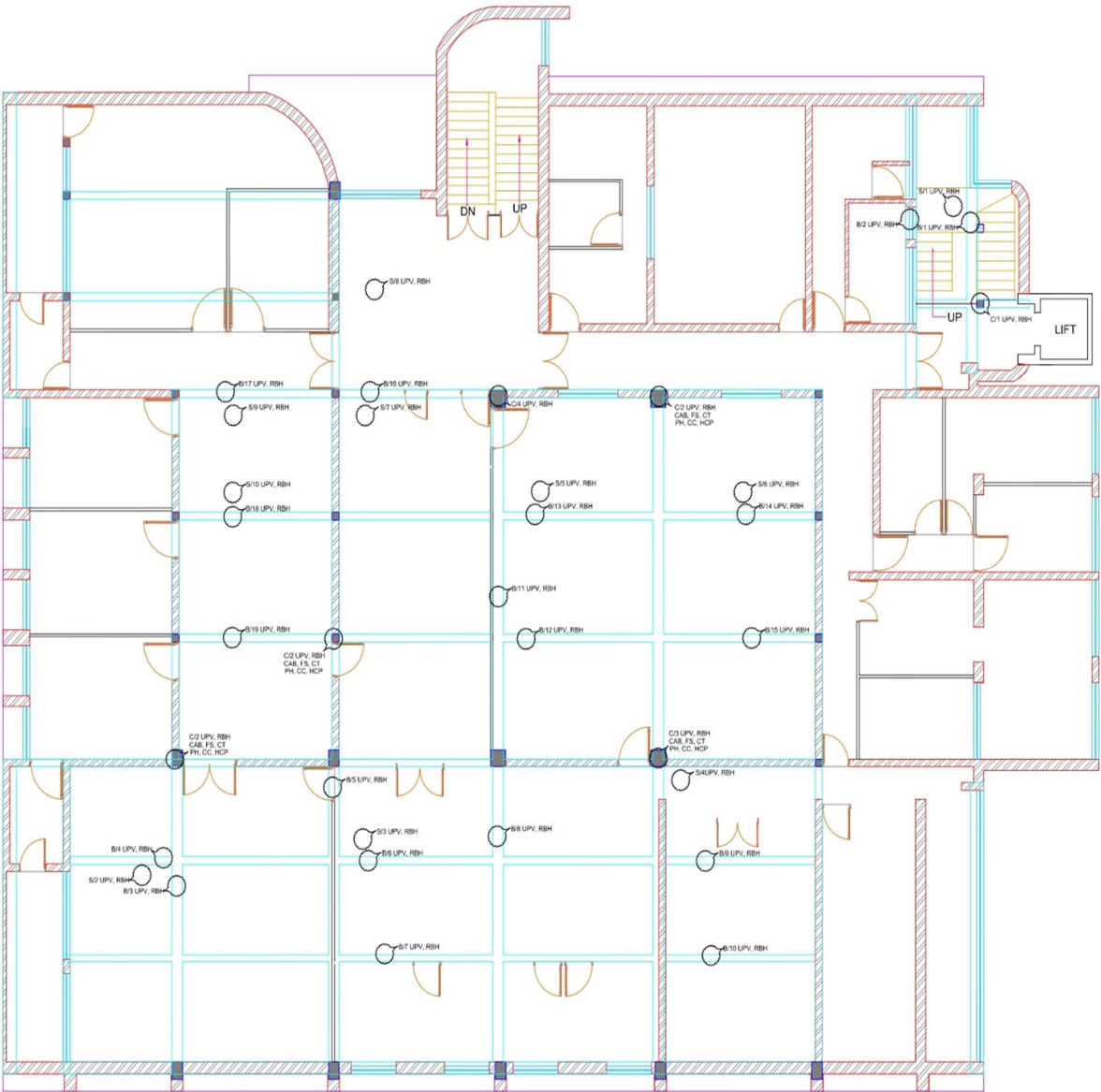
FIRST FLOOR
