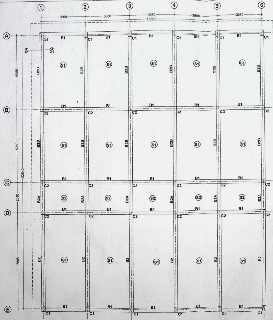
BEAM & SLAB PLAN FOR SECOND FLOOR
