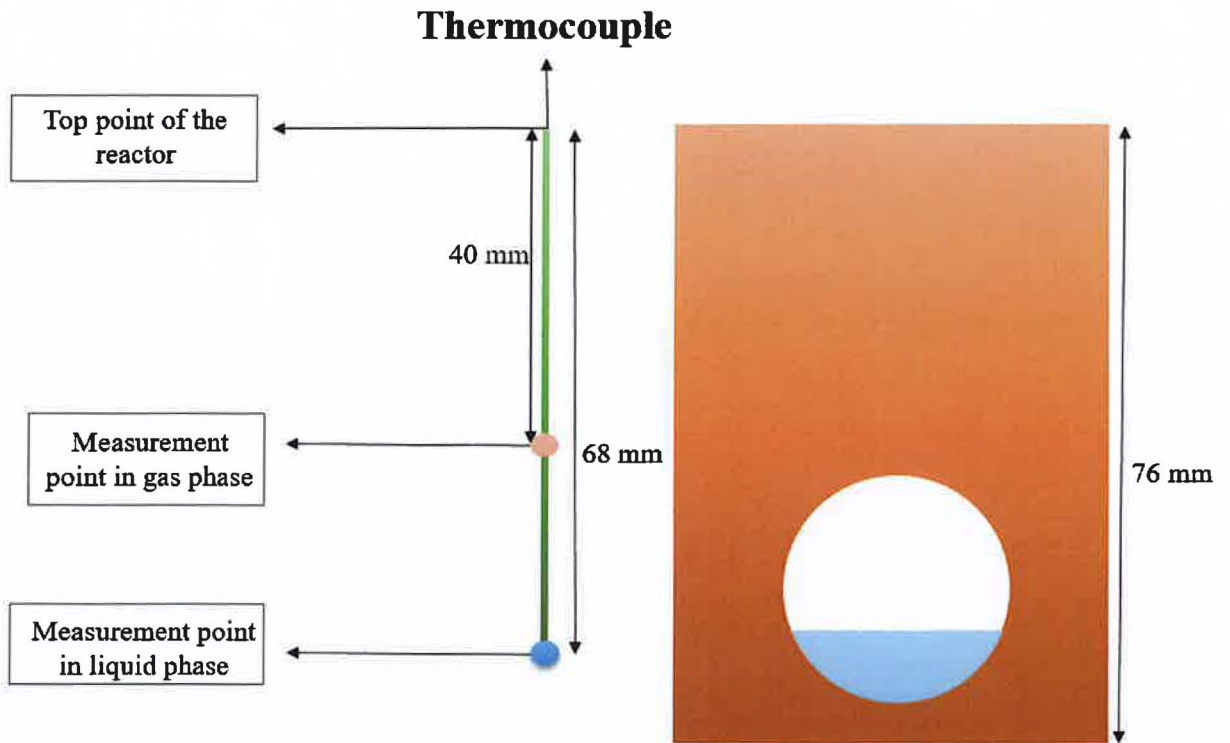
Figure 3. Schematic Representation of Thermocouple Measurement Positions in Gas and Liquid Phases of the Reactor
